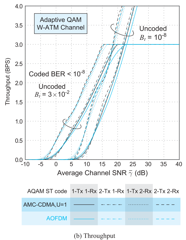
Figure 9 Performance of the concatenated ST block coded and turbo convolutional coded adaptive OFDM and MC-CDMA systems over WATM channel of [4, pp.476]. The uncoded target BER is 3 \times 10^{-2} . The coded BER was less than 10^{-8} for most of the SNR range, resulting in virtually error free transmission. (a) The coded BER becomes higher near the ‘avalanche’ SNR point, when a single antenna was used. (b) The coded adaptive modems have SNR gains up to 7dB compared to their uncoded counterparts achieving a comparable average BER
